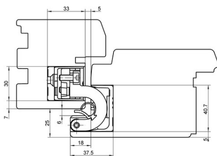
overlap 25 mm
