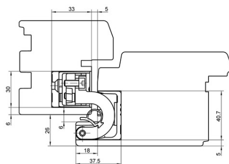
overlap 26 mm
