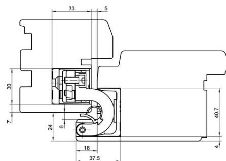
overlap 24 mm
